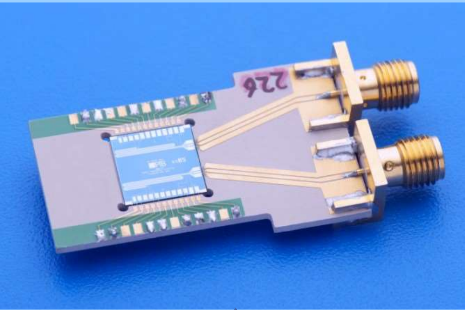
Single chip of the Josephson Arbitrary Waveform Synthesizer (JAWS) mounted in the sample holder. The JAWS is based on pulse-driven Josephson junctions. The 10 mm x 10 mm chip contains two series arrays of 12,000 Josephson junctions each [2018].
